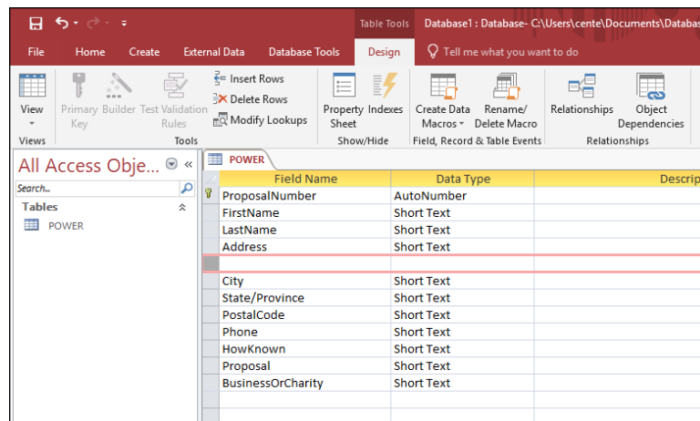
FIGURE 4-8: The table-creation window after opening up space for a second address line.
