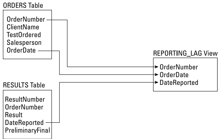
FIGURE 6-2: The REPORTING_ LAG view for the quality-control officer.
