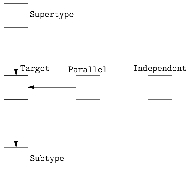
Figure 1: Typedef relationships
