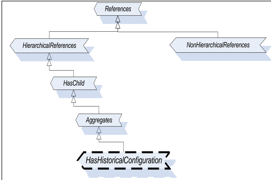
Figure 2 – ReferenceType hierarchy
