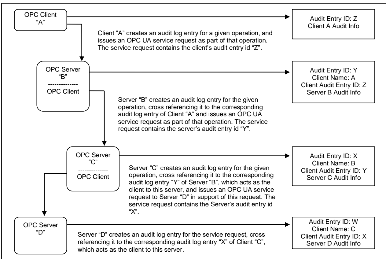
Figure 6 – Aggregating Servers
