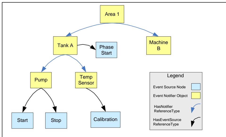
Figure 34 – Event Reference Example
