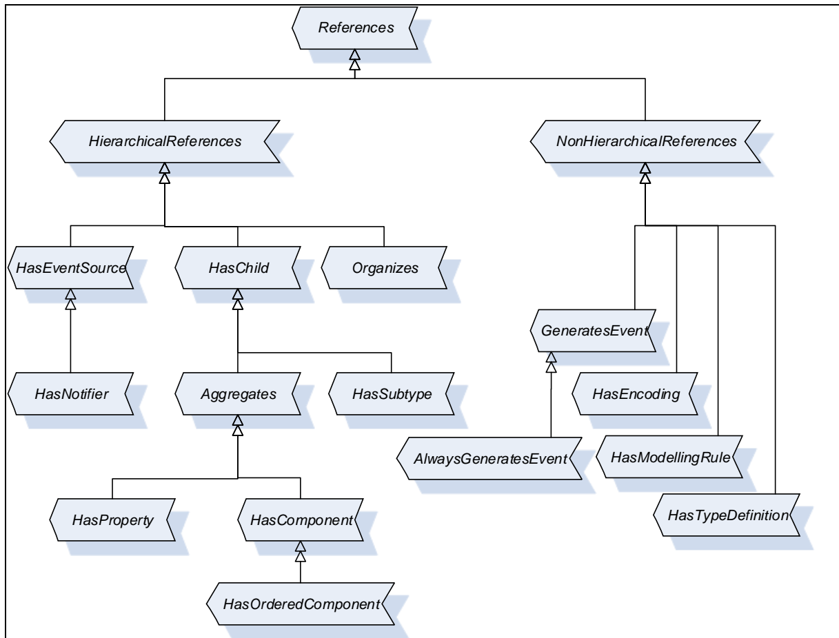
Figure 33 – Standard ReferenceType Hierarchy
