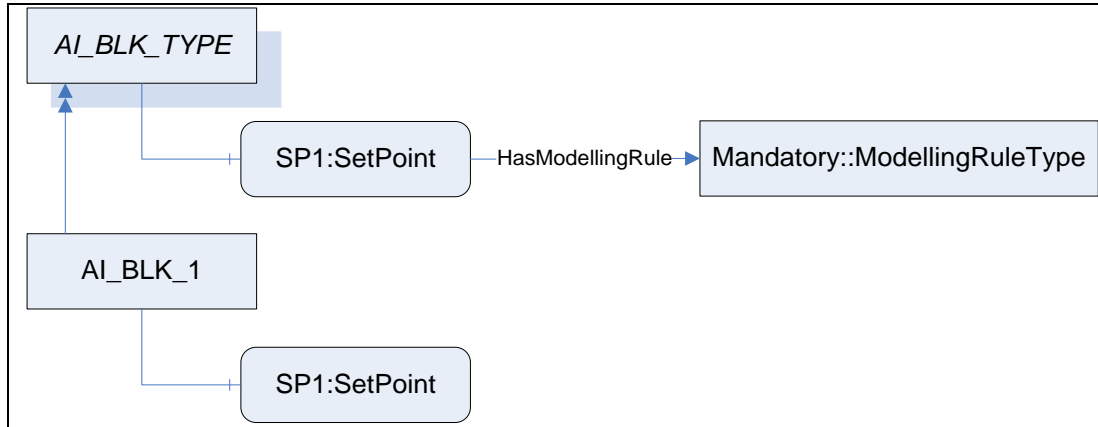
Figure 26 – Use of the Standard ModellingRule Mandatory
