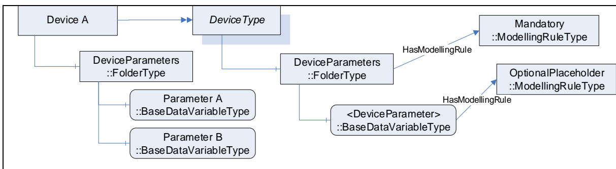
Figure 30 – Example using OptionalPlaceholder with an Object and Variable
