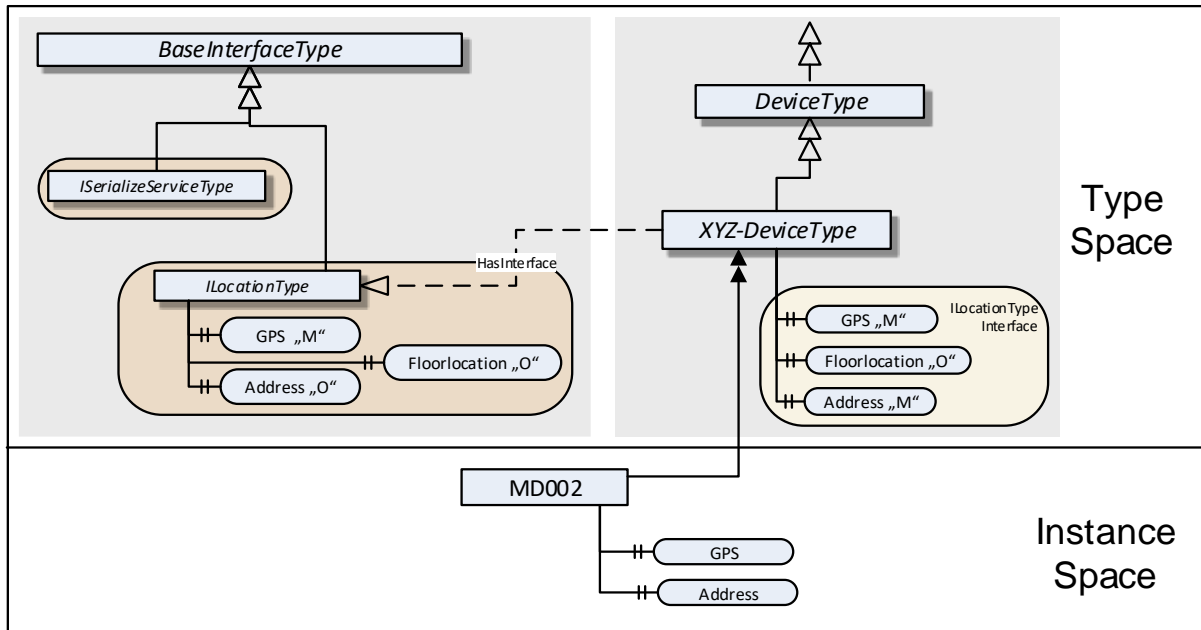
Figure 9 – Example: Interface application to an ObjectType
