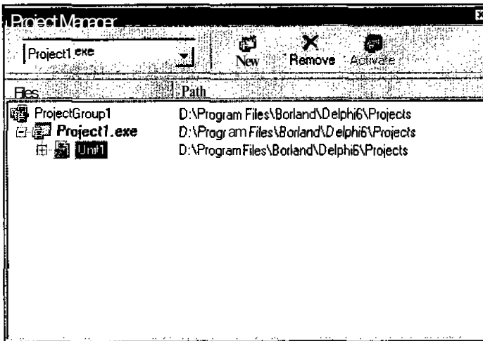
Рис. 1.4. Project Manager
