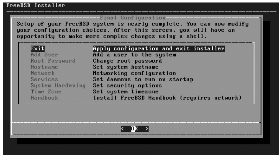
Figure 3-26: Final configuration
