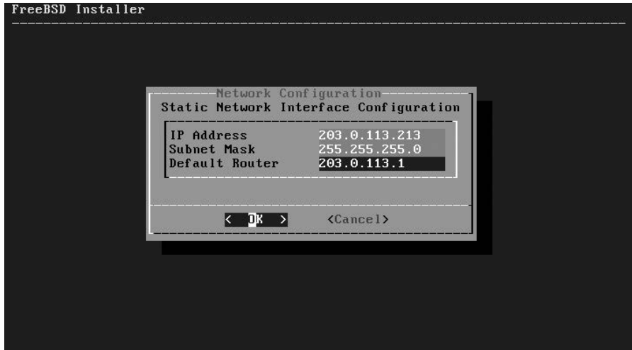
Figure 3-19: Network configuration
