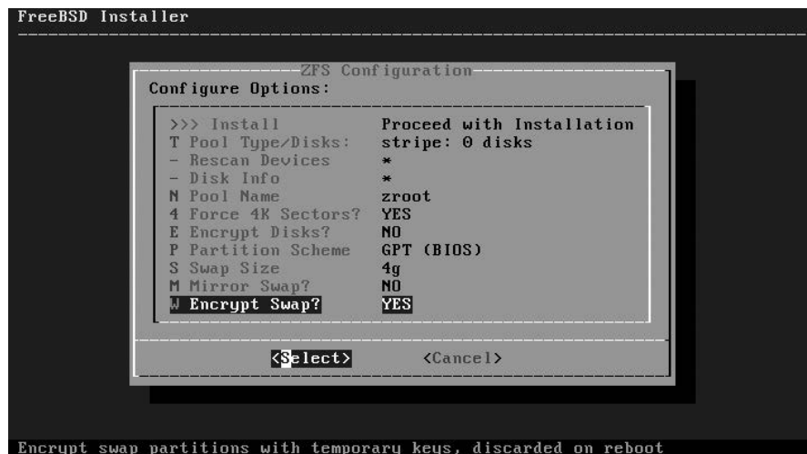
Figure 3-15: ZFS configuration
