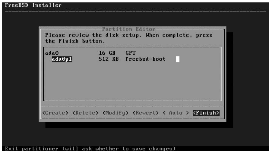
Figure 3-11: Only the boot loader
