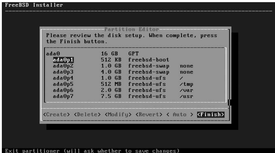
Figure 3-14: Complete custom GPT/UFS partition table
