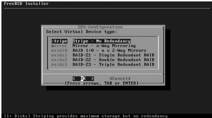
Figure 3-16: Virtual device selection
