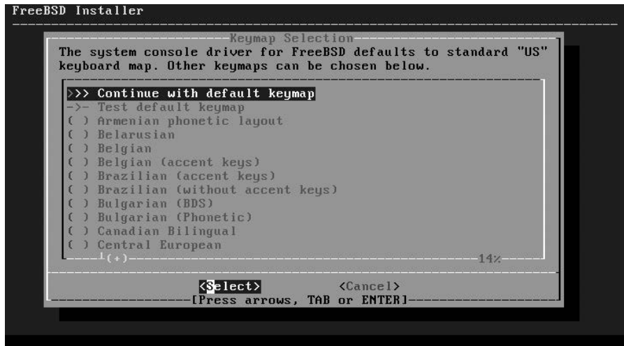
Figure 3-3: Keymap selection
