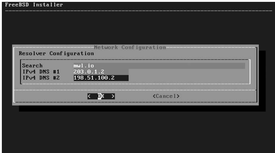
Figure 3-20: Resolver configuration
