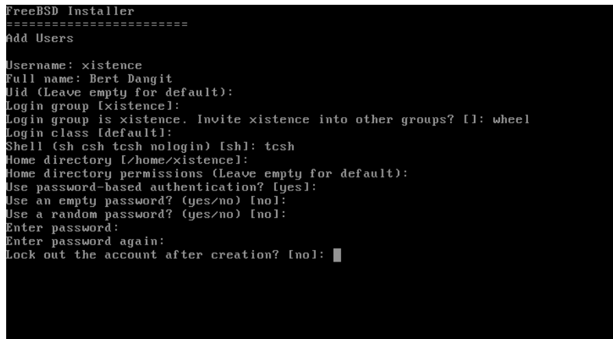
Figure 3-25: Adding a user
