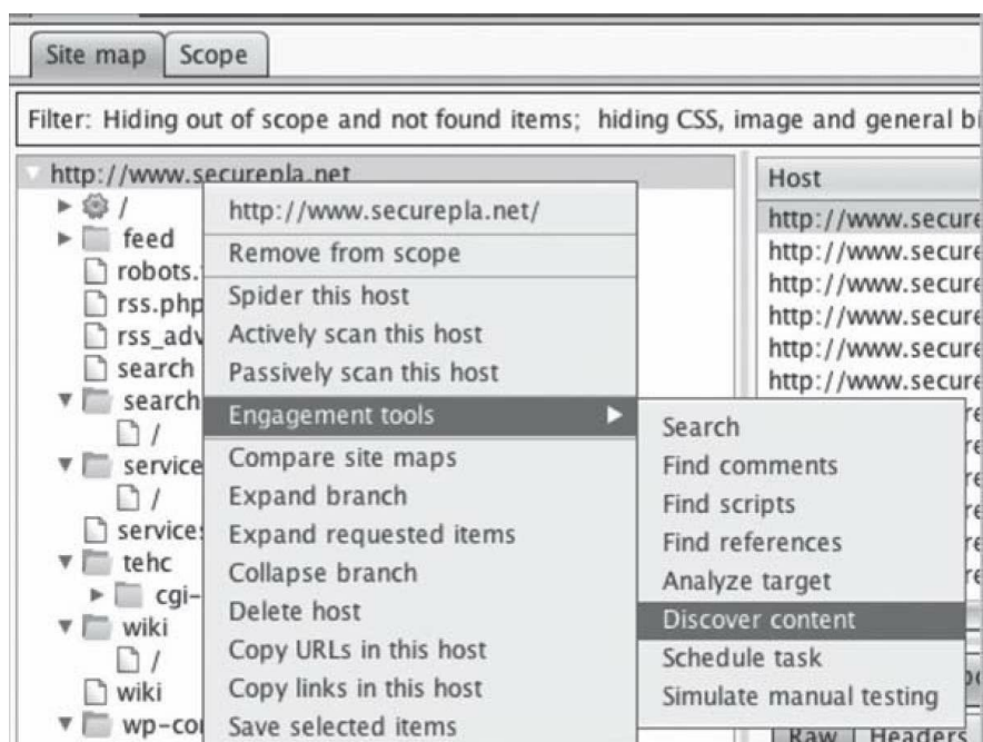
Figure 21 - Discovering Content
