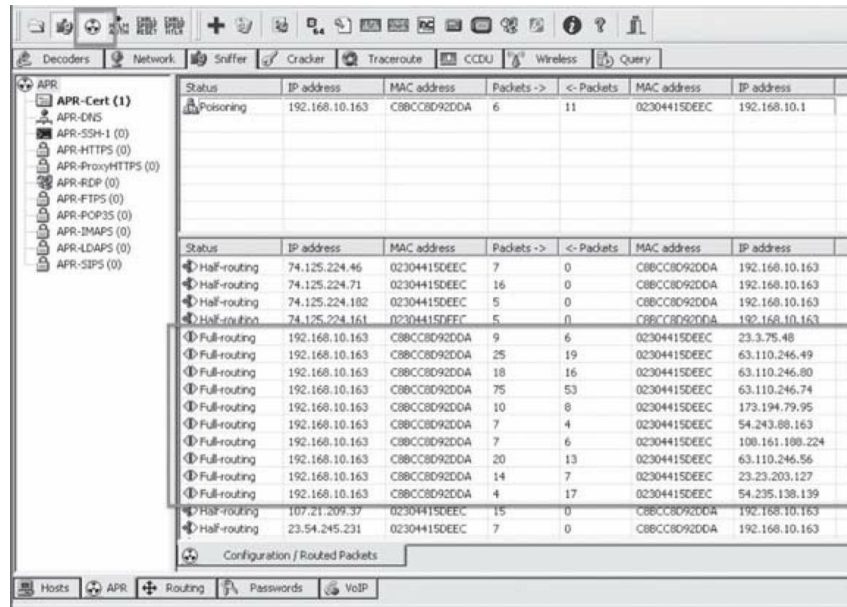
Figure 86 - Successful Poisoning
