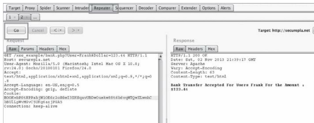
Figure 49 - Executing Burp Repeater
