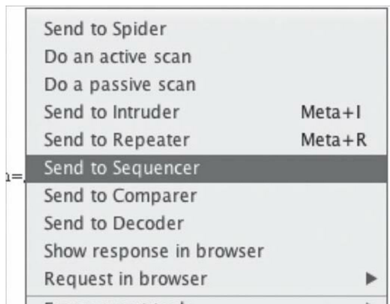
Figure 51 - Sending the Raw Request to Sequencer
