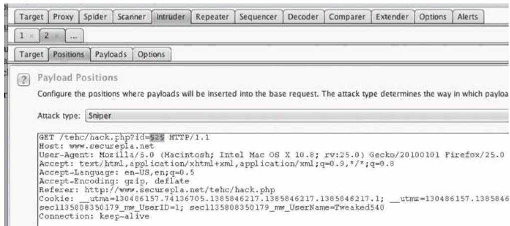
Figure 56 - Burp Payload Positions
