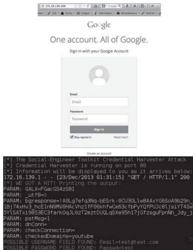
Figure 105 - Spoofed Google Authentication and SET Password Captures
