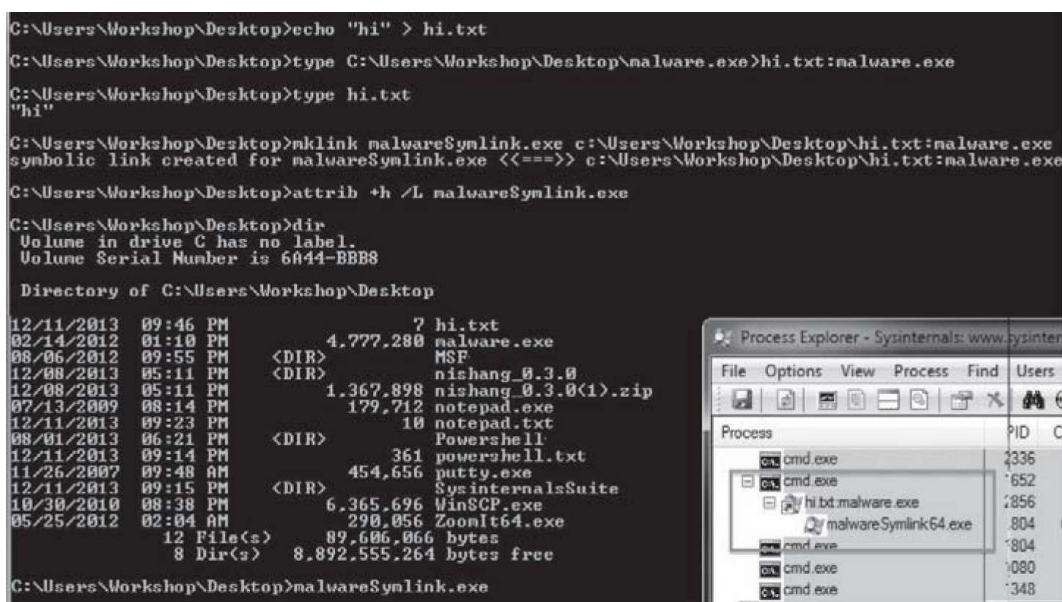
Figure 146 - ADS for Windows 7 and Higher
