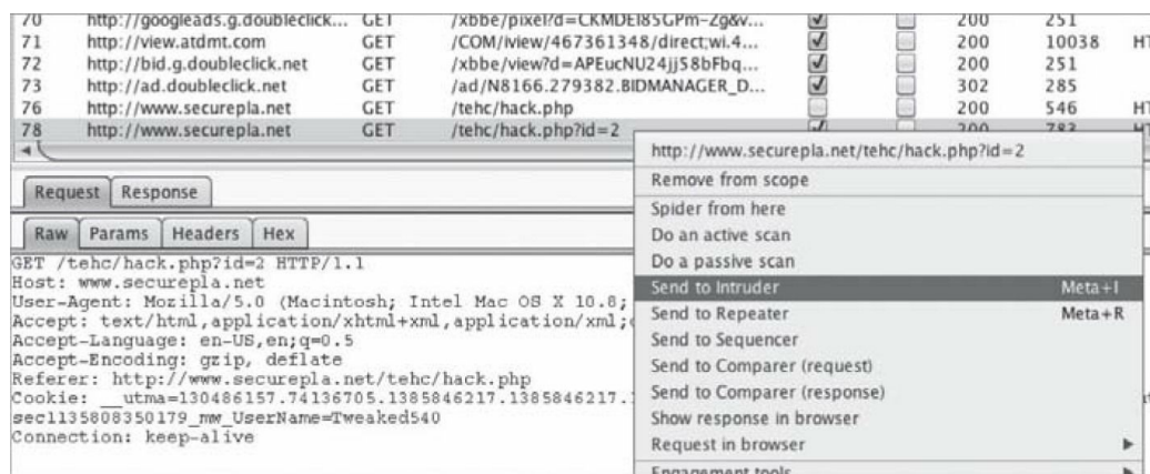
Figure 55 - Sending Request to Intruder
