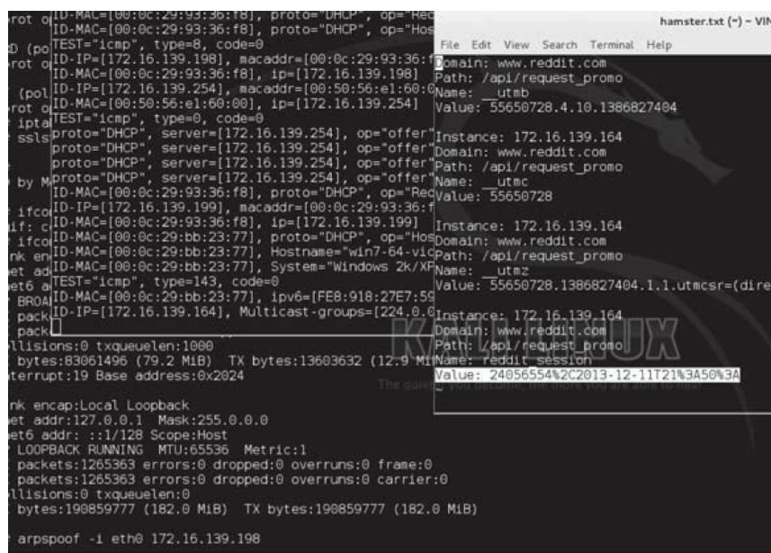
Figure 91 - Hamster Results
