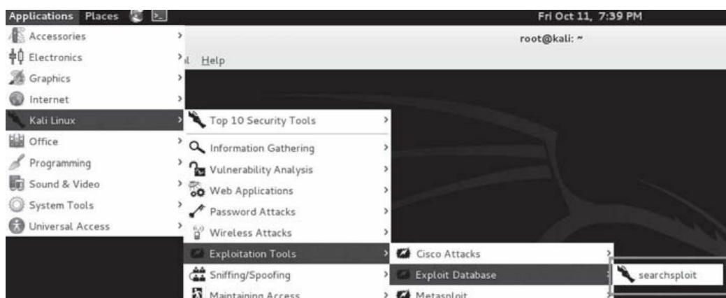
Figure 138 - Searchsploit
