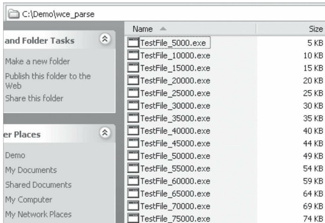
Figure 126 - Evade Output
