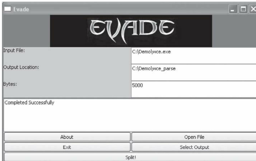
Figure 125 - Evade
