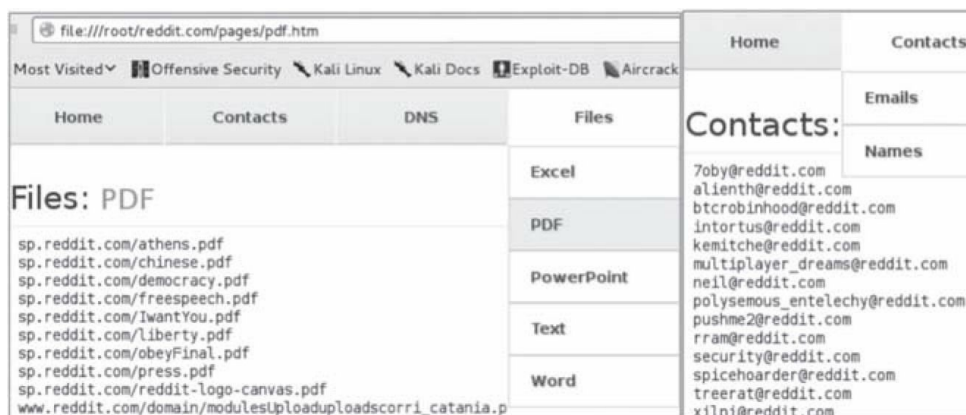
Figure 4 - PDFs and Emails Found Passively
