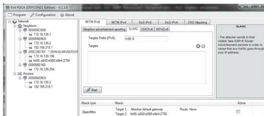
Figure 90 - Evil FOCA SLAAC
