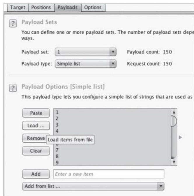
Figure 57 - Burp List
