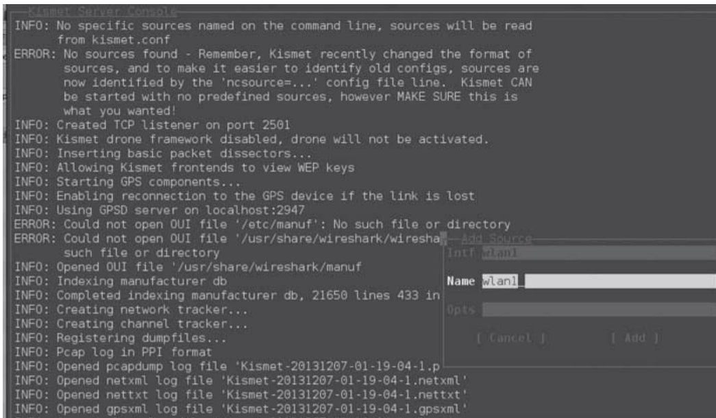
Figure 115 - Kismet Configuration
