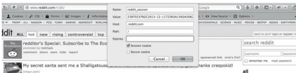
Figure 92 - Replacing Cookies
