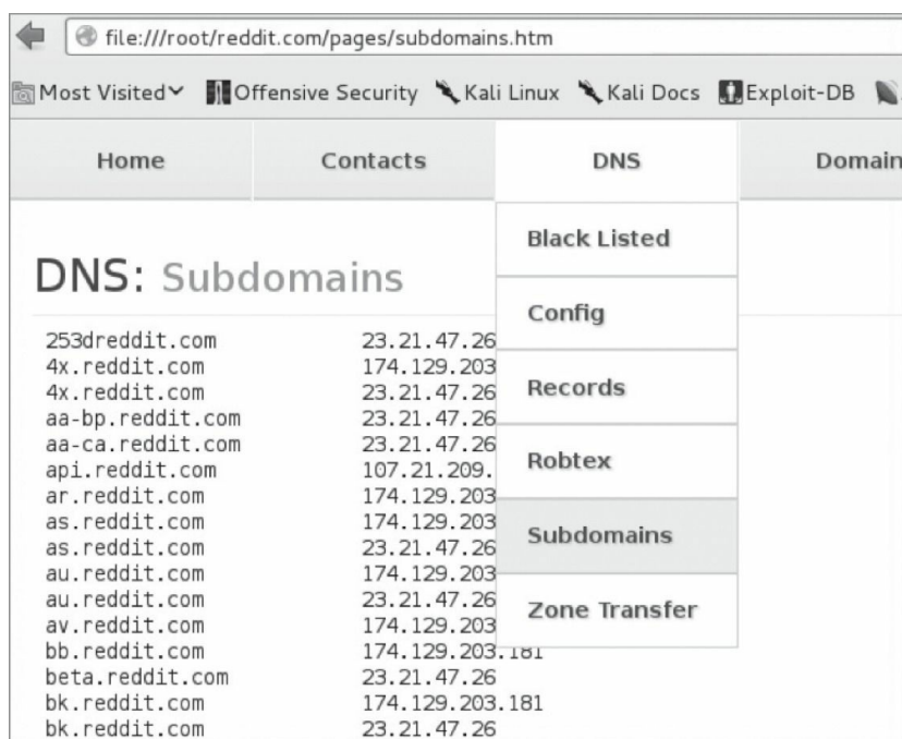
Figure 3 - Subdomains for Reddit
