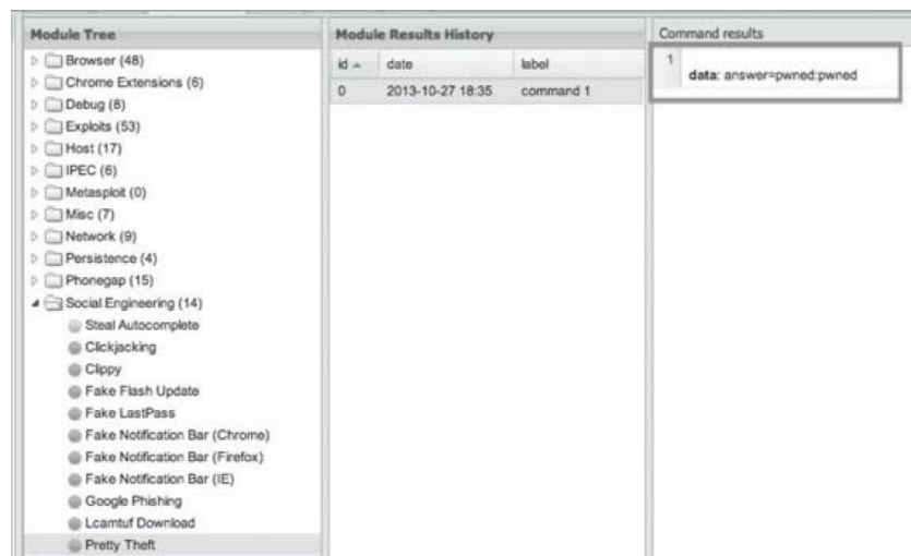
Figure 44 - Petty Theft Results
