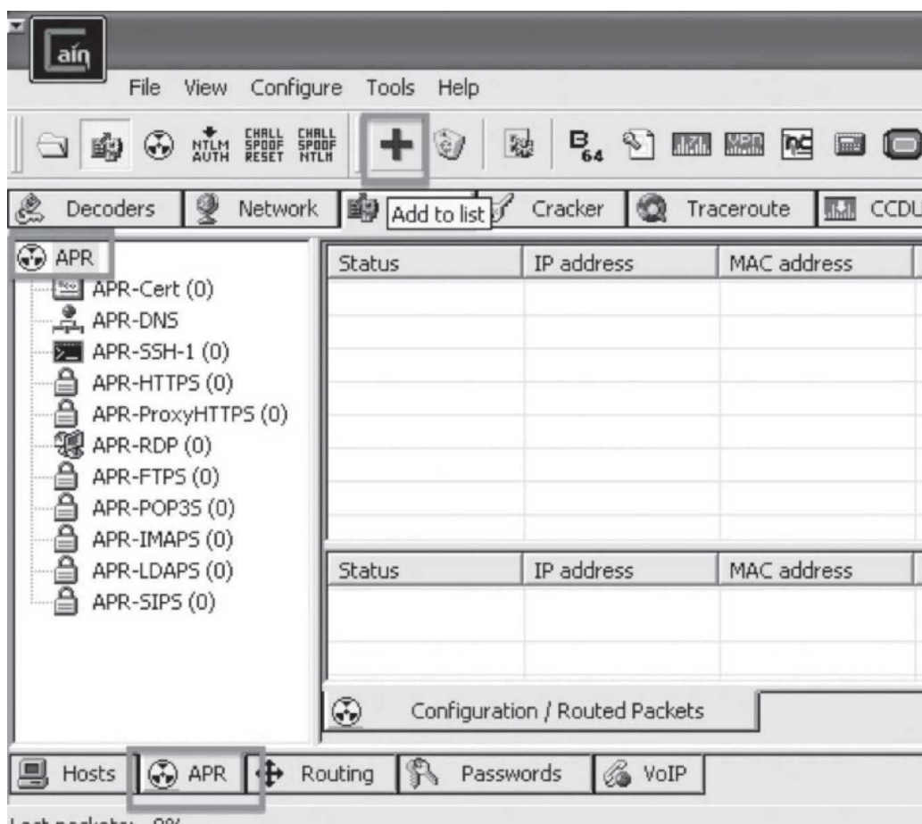
Figure 84 - APR List
